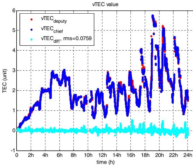
Figure 8. VTEC profiles of two spacecraft receivers.
