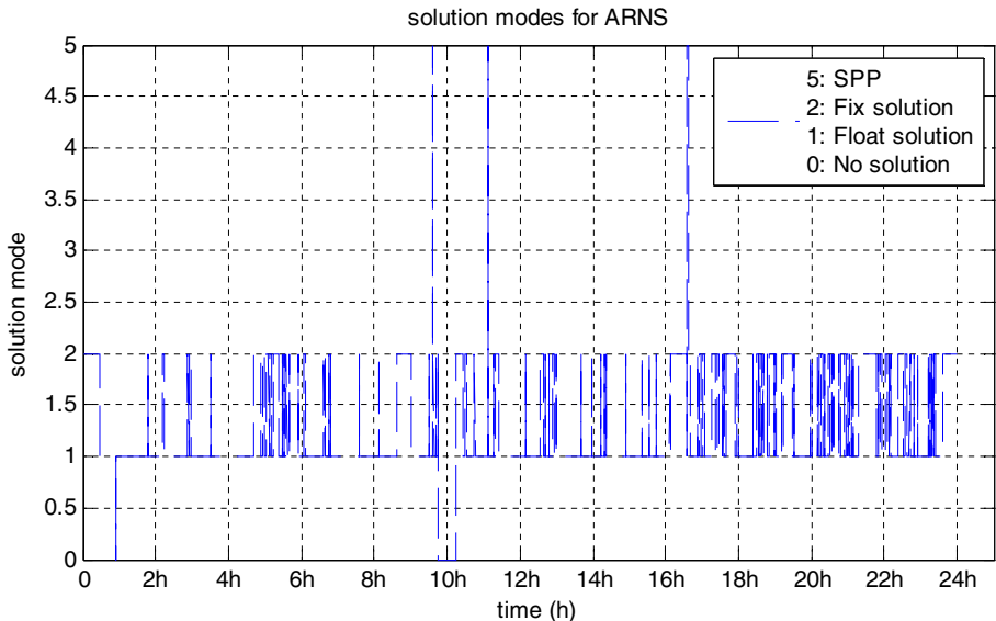
Figure 9. Relative navigation solution modes for the ARNS with fixed ambiguity feedback.
