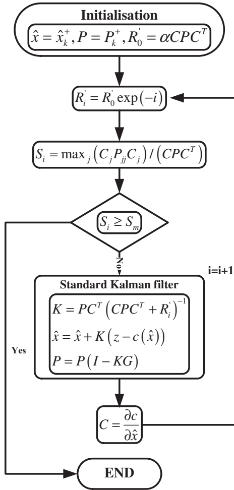
Figure 1. SCKF algorithm.
