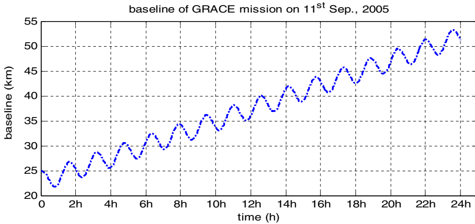
Figure 4. Inter-satellite separation for the GRACE mission.
