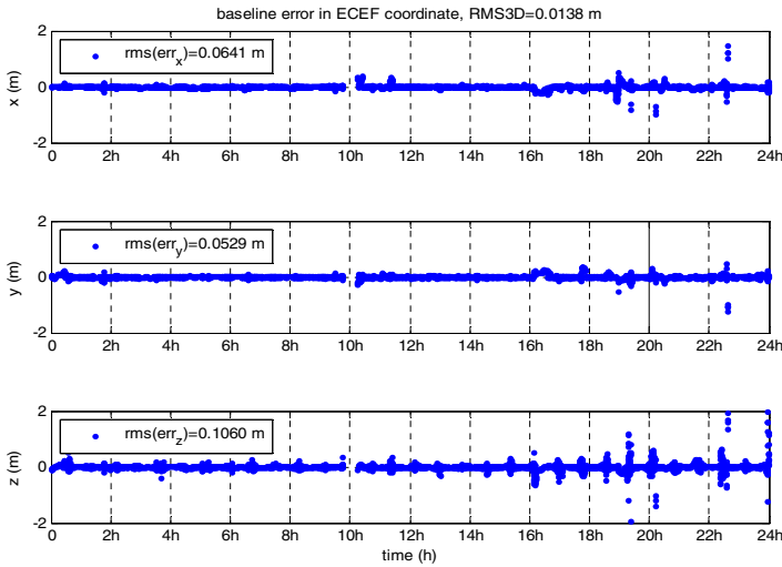
Figure 7. Baseline estimation errors for SCKF-based ARNS.
