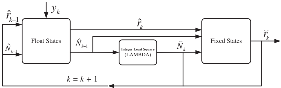
Figure 2. Fixed ambiguity feedback scheme for the GPS stand-alone relative navigation system.
