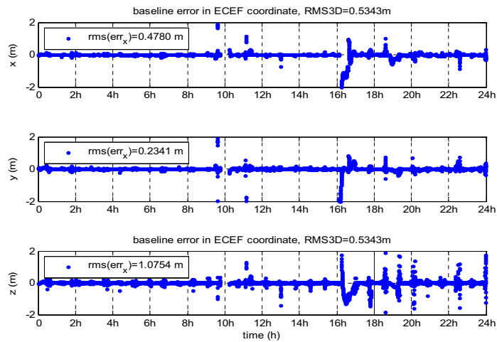
Figure 6. Baseline estimation errors for GPS stand-alone solutions.
