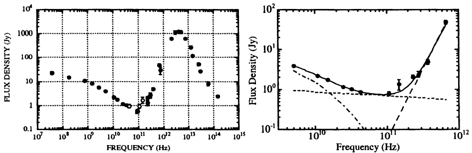
Figure 2. Left: Integrated spectral energy distribution of M82. Our data is shown by open circle. Right: Spectral fit with dust (dashed line), free-free (dotted line) and synchrotron (dot-dashed line) emissions. Synchrotron emission is modeled by second order polynomial on logarithmic plot to incorporate with the synchrotron loss. Plotted data are only from single dish mapping observations and low frequency VLA observations.
