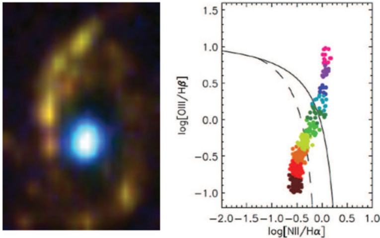
Figure 1. An example of data products produced in the S7 survey. The Left-hand panel is an image of NGC 6890 in H \alpha (red), [N II] \lambda 6584 (green) and [O III] \lambda 5007 (blue), boxcar smoothed over one arc sec. The H II regions appear reddish or gold depending on their excitation, and trace out the spiral arms, while the nucleus and the ENLR appears blue. On the right-hand panel we show the BPT diagram for the individual spaxels, colour coded according to the angular distance from the nucleus. This forms a tight mixing sequence between pure AGN line ratios (magenta) and pure HII region emission (brown). Compare e.g. Dopita et al. (2014); Davies et al. (2014a).
