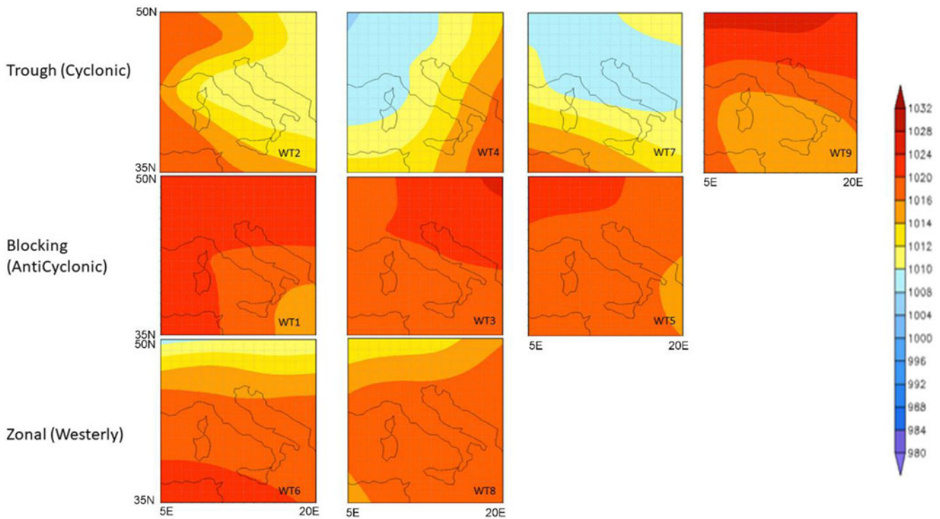
Fig. 3. Colour online. Circulation type classification for Italy based on principal component transversa (PCT) methods for precipitation.
