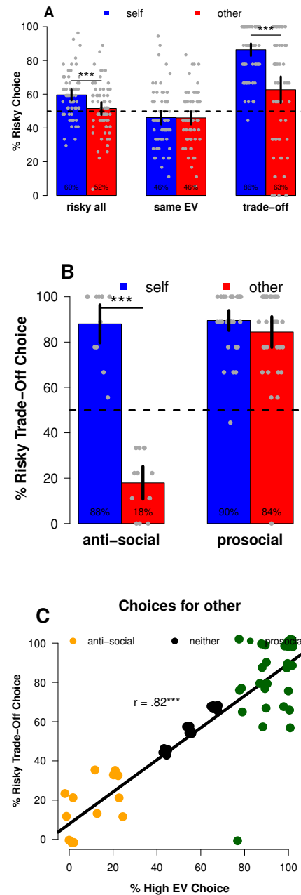
FIGURE 4: (A) Mean percentage ( \pm 95\% CI) of risky choices for self and other in all choice situations with different ranges (choice situations 1–9, left) and separately for those with the same expected value (1–6, middle) and those with a risk-return trade-off (7–9, right). Grey points represent individual participants with horizontal jitter. (B) Mean percentage ( \pm 95\% CI) of risky choices for self and other with a risk-return trade-off (7–9), split by participant classification. (C) Percentage of risky choices for others in the risk-return trade-off choices (7–9) correlated with the percentage of dominant choice for other in classification trials (19–21), where colors illustrate the classification scheme applied and both vertical and horizontal jitter were used. *** = p < .001 .
