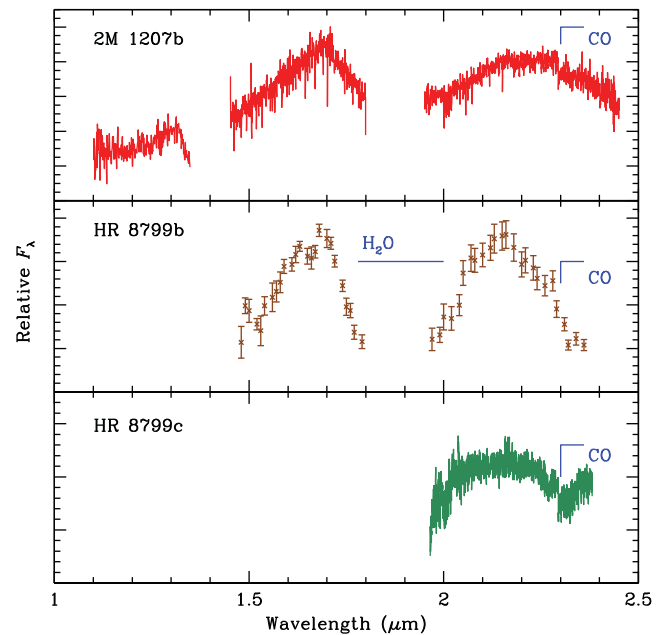
Figure 10. Spectra of the direct imaged planets (or planetary mass objects) 2M 1207b (Patience et al. 2010), HR 8799b (Barman et al. 2011a) and HR 8799c (Konopacky et al. 2013). The CO bandhead at 2.3 \mu\text{m} is apparent in all three objects as well as \text{H}_2\text{O} absorption at \sim 1.9 and \sim 1.4 \mu\text{m} .
