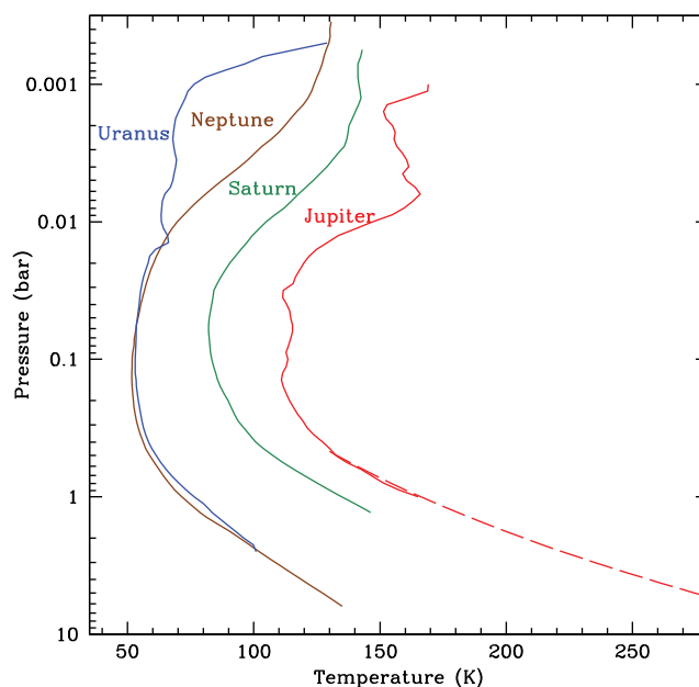
Figure 8. Temperature profiles of the Solar system giant planet atmospheres from Voyager radio occultation measurements (Lindal 1992), and from the Galileo probe for Jupiter (dashed line – Seiff et al. 1998).
