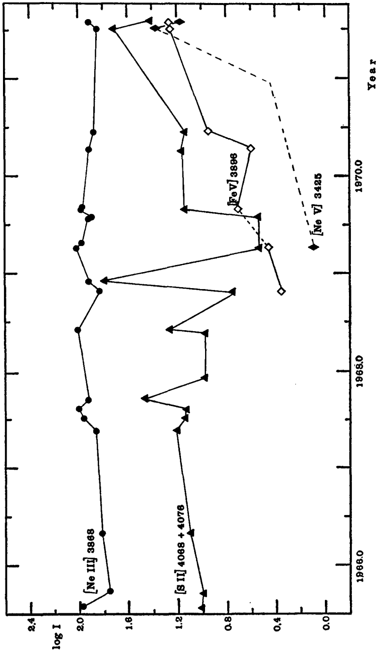
Fig. 5: Variation in log I for [NeIII], [NeV], [SII] and [FeV]. \log I(H\beta) = 2.00 .
