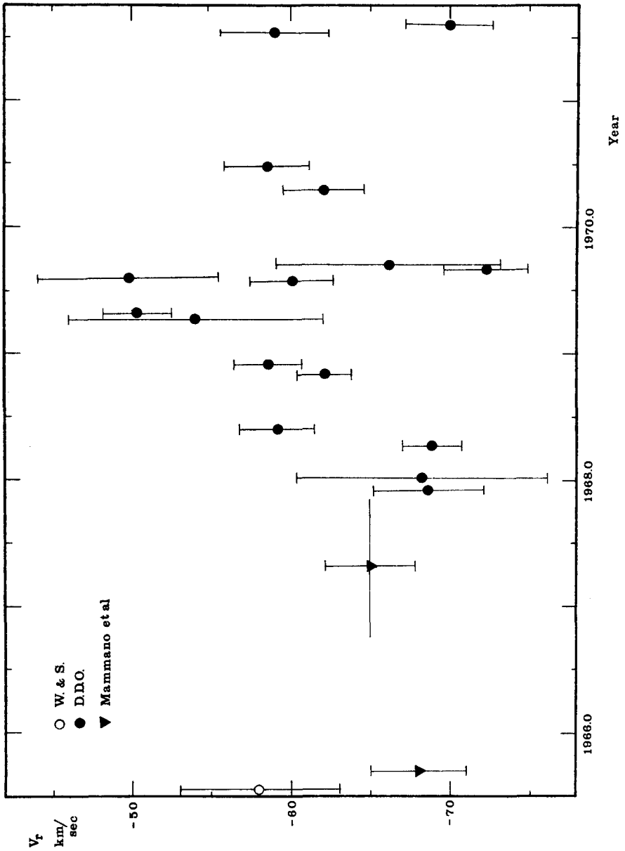
Fig. 7: Radial velocities of V 1016 Cygni. The bars represent standard errors of the mean.
