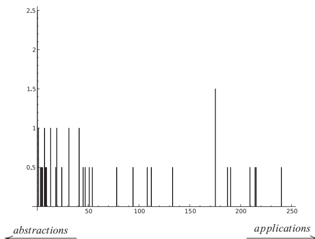
Fig. 12. Distribution of simply typable closed \lambda -terms of size 30 on 250 segments on the horizontal axis, percentage (0%–2.5%) of typable closed \lambda -terms in segments on the vertical axis.
