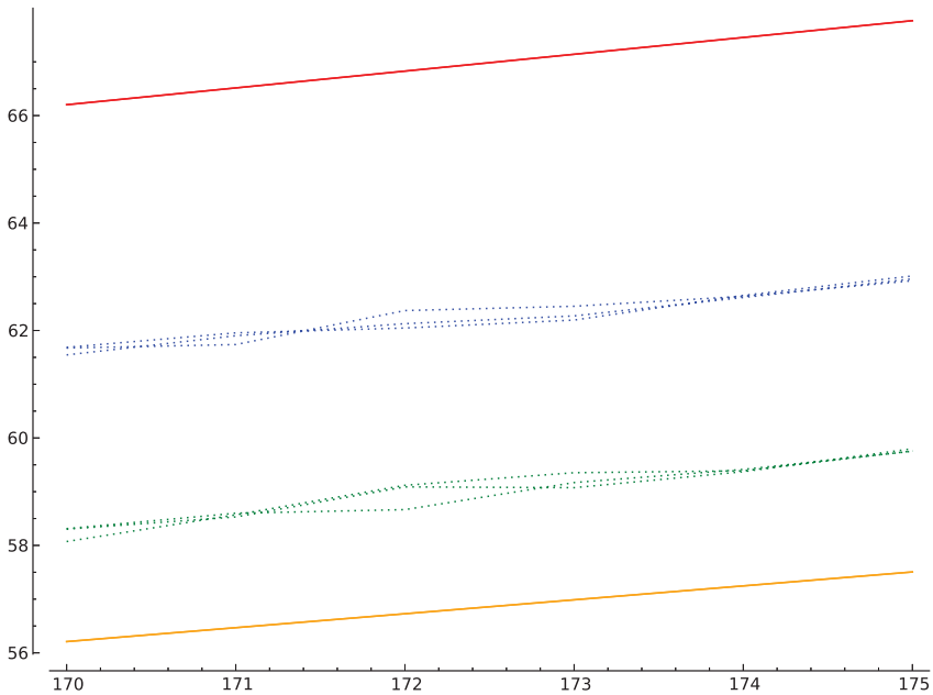
Fig. 9. (Colour online) Magnification of Figure 8 between n = 170 and n = 175 .
