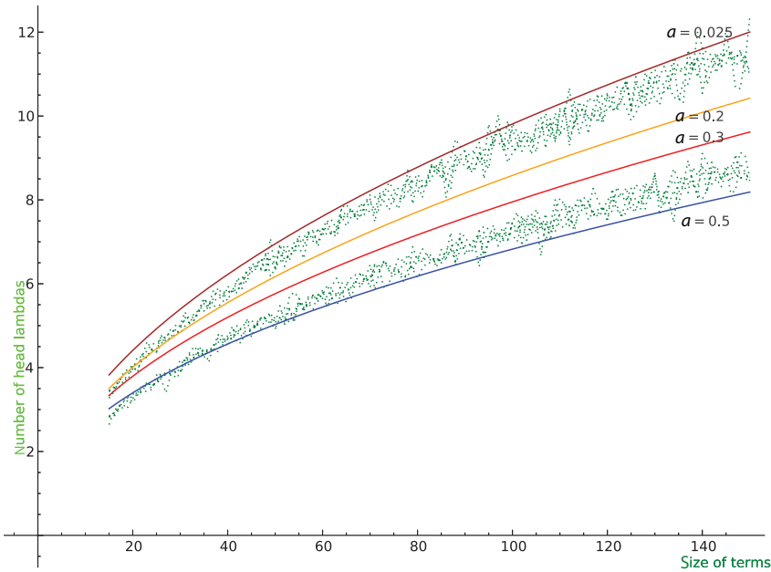
Fig. 10. (Colour online) Bottom: Average number of head \lambda s per closed term. Top: Average number of head \lambda s per closed normal form. In-between: Curves \sqrt{\frac{n}{\ln(n)^a}} for a = 0.025, 0.2, 0.3, 0.5 .
