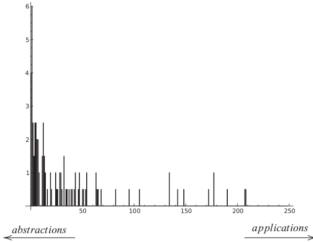
Fig. 13. Distribution of simply typable closed normal forms of size 25 on 250 segments on the horizontal axis, percentage (0%–6%) of typable closed normal forms in segments on the vertical axis.
