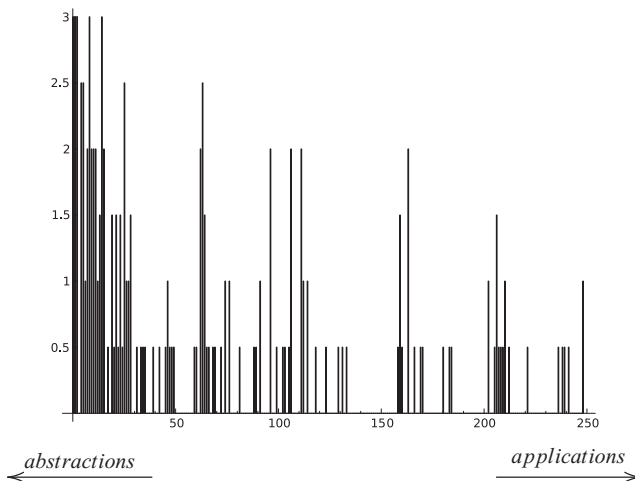
Fig. 11. Distribution of simply typable closed \lambda -terms of size 25 on 250 segments on the horizontal axis, percentage (0%–3%) of typable closed \lambda -terms in segments on the vertical axis.
