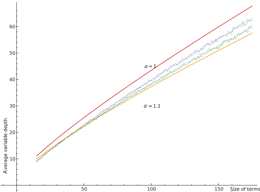
Fig. 8. (Colour online) From top to bottom: Curve \frac{2n}{\ln(n)} , average variable depth for closed terms, average variable depth for closed normal forms and curve \frac{2n}{\ln(n)^{1.1}} .
