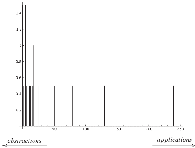
Fig. 14. Distribution of simply typable closed normal forms of size 30 on 250 segments on the horizontal axis, percentage (0%–1.45%) of typable closed normal forms in segments on the vertical axis.
