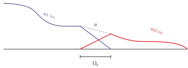
Fig. 3. Example of solution in one dimension. The solution u is the sum of u_1 and u_2 on the blending zone. Homogeneous Dirichlet conditions are imposed on the border of the blending zone following Eqn (21).
