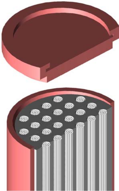
FIG. 2. The proposed canister for Lithuanian SNF disposal (reproduced from Poskas et al. , 2006).
