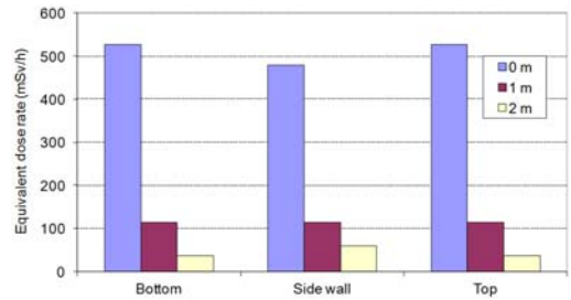
FIG. 3. The total equivalent dose-rate values on the copper canister surface and at distances of 1 and 2 m (reproduced from Poskas et al. , 2006)
