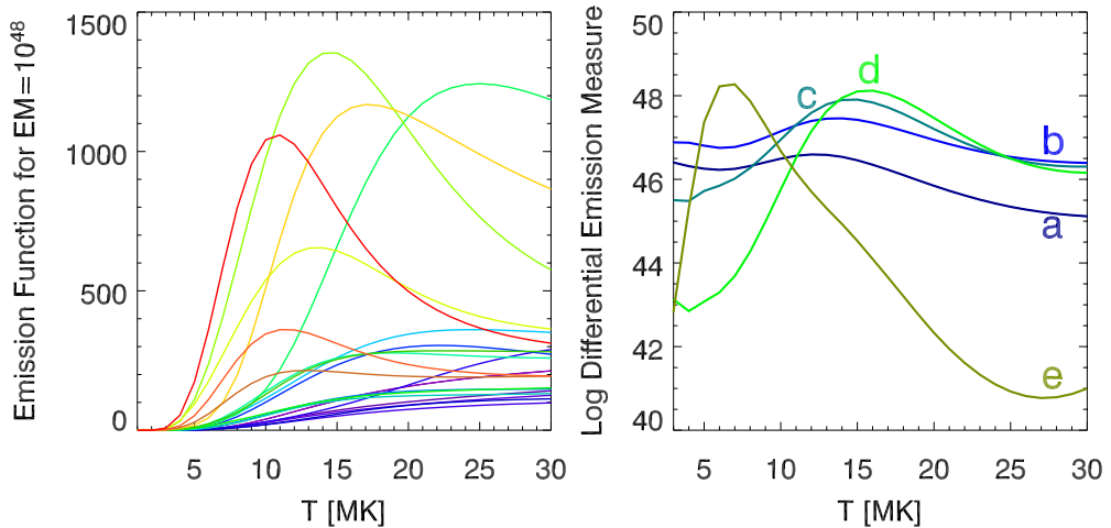
Figure 1. L : The theoretical emission functions (in photons \text{cm}^{-2} \text{s}^{-1} , lines plus continuum included) used in the calculations; R : Example DEM curves for 5 time intervals (a, b, c, d - rise phase, e - late decay) for the 7 January 2003 flare.
