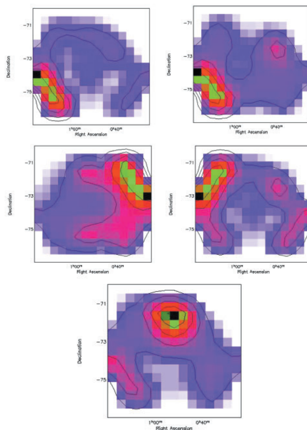
Figure 4 Clockwise from the top left: distribution of the metallicity that corresponds to the maximum probability for a star-formation rate equivalent to a mean age of 2.0, 3.9, 6.3, 8.7 and 10.6 Gyr for C stars across the SMC. Contours are at: 0.7, 0.8, 0.9, 0.94 and 0.98 expressed in terms of Z (Cioni et al. 2006b).
