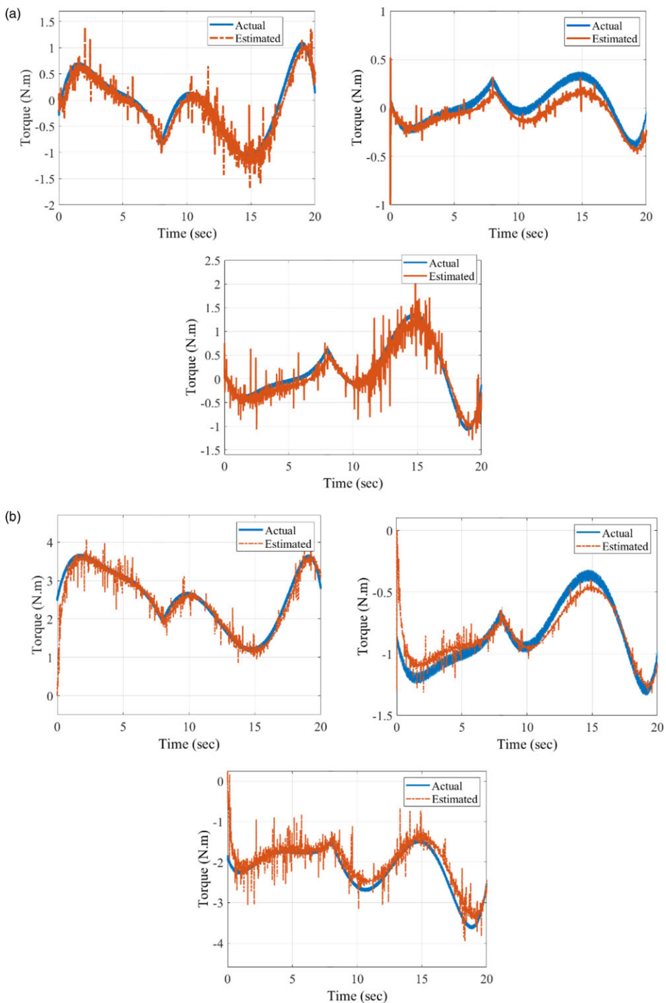
Figure 21. Time histories of actual resistance torque \tau_o and estimated resistance torque \xi_o in (a) case 1 and (b) case 2.
