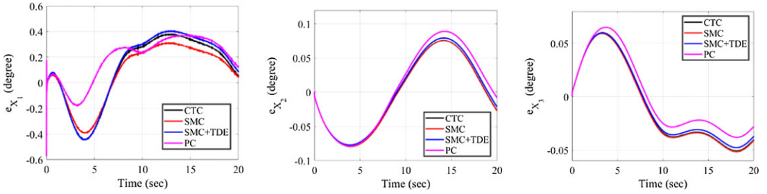
Figure 14. The closed-loop tracking performance of the RSPM for different controllers in the presence of lower bound uncertainties.
