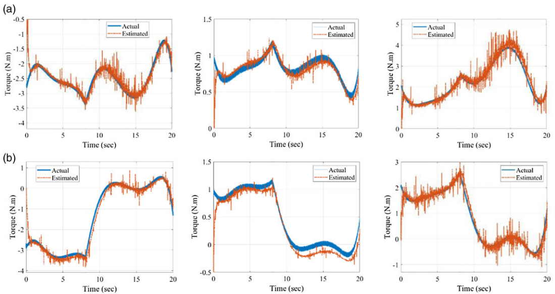
Figure 23. Time histories of actual resistance torque \tau_\rho and estimated resistance torque \xi_\rho in (a) case 3 and (b) case 4.
