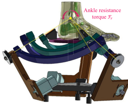
Figure 3. Applied ankle resistance torque \mathcal{F}_r to the robot in Cartesian space.
