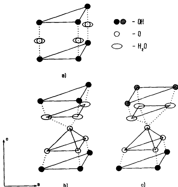
Figure 1. Arrangement of water molecules and carbonate (a) or sulphate (b and c) in the interlayers of P- (a and b) and O-types (c). OH are hydroxyl groups of brucite-like layers; O are oxygens of interlayer anions. In carbonate varieties, water molecules occupy the same crystallographic sites as oxygens of the anion. In sulphate varieties, triangles of water molecules together with a \text{SO}_4 -pyramid construct dumbbells. Dotted lines represent H-bonding net in the interlayers.
