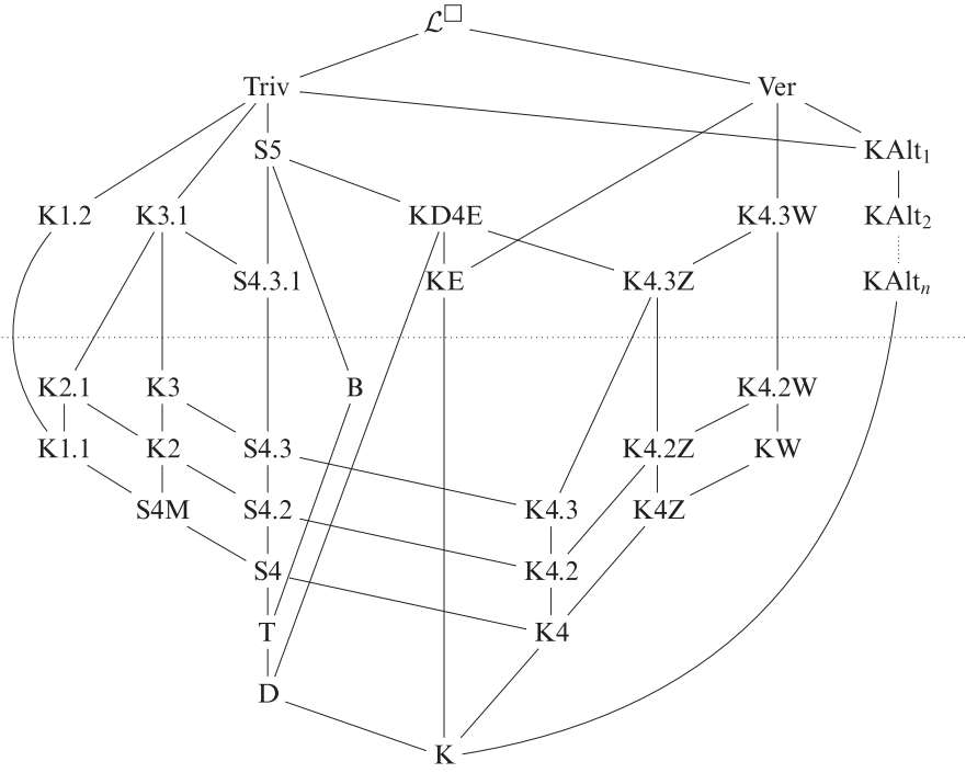
FIGURE 1. The axiomatizability boundary (dotted) among some finitely axiomatized normal modal logics.
