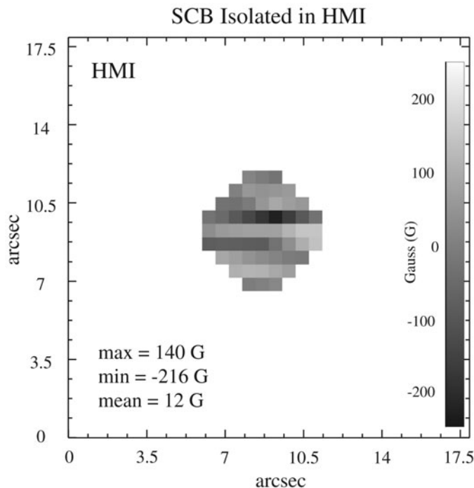
Figure 2. The SCB highlighted in Figure 1 isolated in HMI. The boundary of the SCB is determined by the flux in H\alpha and then overlaid on the coincident photospheric magnetogram to isolate the magnetic signature of the SCB.
