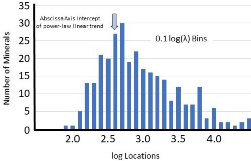
Figure 5. Frequency distribution of those mineral-location pair data that plot along the abscissa axis of Figure 3B in 0.1 \log_{10}(\lambda) bins, illustrating the highly skewed nature of the dispersion of commonly occurring minerals. Importantly, the power-law trend calculated in Figure 4A intersects the abscissa axis within one bin of the modal value of this distribution.
