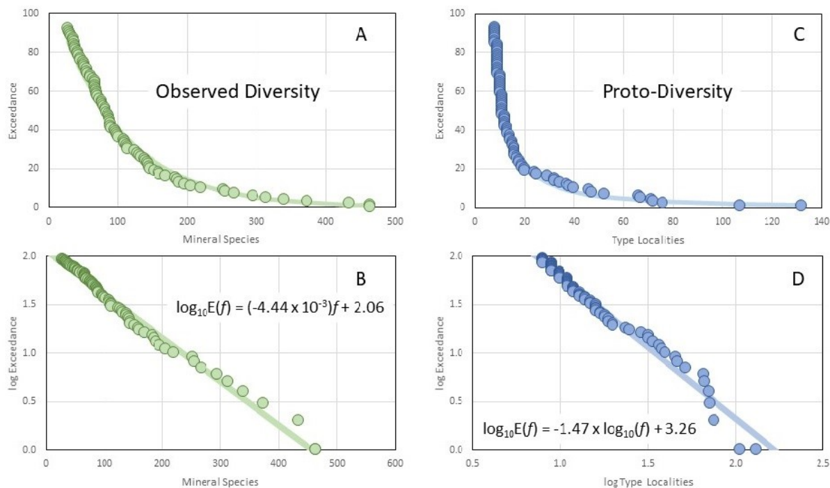
Figure 1. Mineral hotspots are defined as those locations, or groups of sublocations clustered in close geographic proximity, that are characterized by either an abundance of mineral species (observed diversity) or an abundance of minerals first discovered at that location (proto-diversity). Using the formulation E(f) where E is the number of locations with more minerals than the value f , known as the exceedance value, data are displayed from the most mineral-rich hotspots (Mindat.org). The observed diversity exceedance distribution follows an exponential curve (A) [ \log_{10} E(f) = (-4.44 \times 10^{-3})f + 2.06 ] (B). The concavity of the proto-diversity curve (C) is much greater than the observed diversity data (A) such that the proto-diversity data define a power-law exceedance relationship [ \log_{10} E(f) = -1.47 \times \log_{10}(f) + 3.26 ] highlighting the extreme scarcity of locations rich in previously unknown minerals (D).
