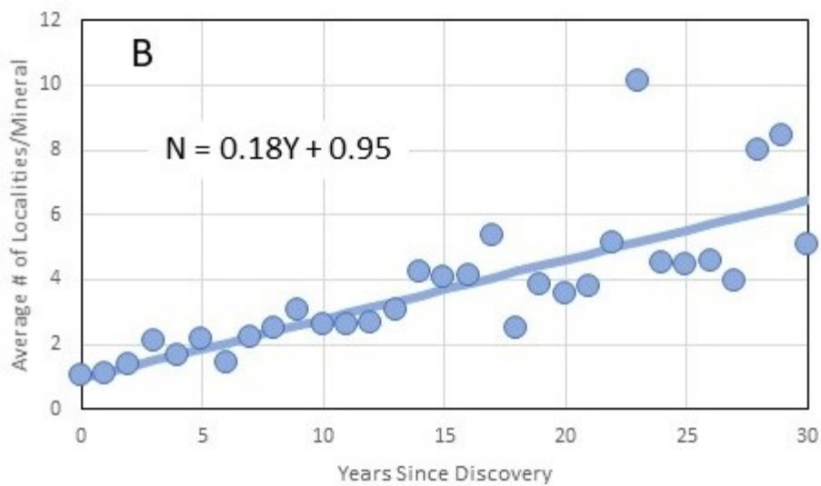
Figure 6. When first discovered, new mineral species are typically exclusively endemic to their type locality. Over time, most minerals are subsequently identified in other locations. The percentage of minerals from a year in the past that are known only from their type locality decreases with increasing time describing an exponential curve [ \%M = 10^{(-0.023Y - 0.01)} ] (A). Similarly, the average number of known locations for minerals increases with time since their discovery following a linear function [ N = 0.18Y + 0.95 ] (B) such that an additional location is found, on average, every 5.5 years ( 1/0.18 ). The y-intercept value of 0.95 confirms the notion that most minerals are initially known from only one location.
