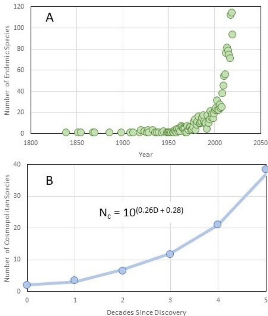
Figure 7. Most minerals that are known from only their type locality have recently been discovered. However, there are some species that were first discovered in the past that remain endemic to their type locality for extended periods (A). Conversely, some recently discovered minerals are now known from a relatively large number of locations. The number of cosmopolitan species (here defined as 50 or more mineral-location pairs) increases with time. When aggregating the number of such species per decade, this increase follows an exponential curve [ N_c = 10^{(0.26D + 0.28)} ](B).
