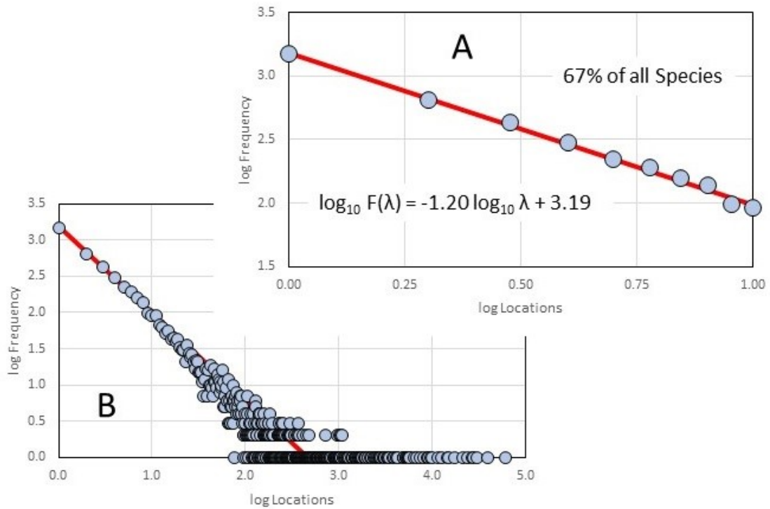
Figure 4. Utilizing the community-sourced database Mindat.org to harvest mineral-location pairs for all IMA accepted species in January, 2021, a power-law relationship between the number of species and the number of locations from which they are known is observed with minerals known from 10 or less locations [ \log_{10} F(\lambda) = -1.20 \log_{10} \lambda + 3.19 ] which accounts for more than 2/3 of all known species (A). This power law relationship is found to extend over several orders of magnitude with increasing dispersion around the regression as the logarithm of location frequency increases (B).
