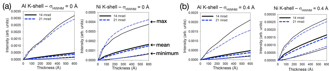
Figure 2. Simulated signal for Ni_3Al_{\langle 100 \rangle} . (a) Maximum, mean, and minimum signals plotted without (a) and with (b) incorporating the finite effective source size.
