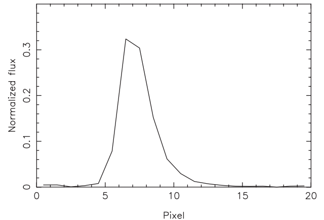
Figure 1 5105.541\text{ \AA} Cu emission line extracted from fibre 1 of a CCD1 calibration lamp observation. The emission line shows an asymmetry towards higher wavelengths that accounts for \sim 30\% of the total signal.
