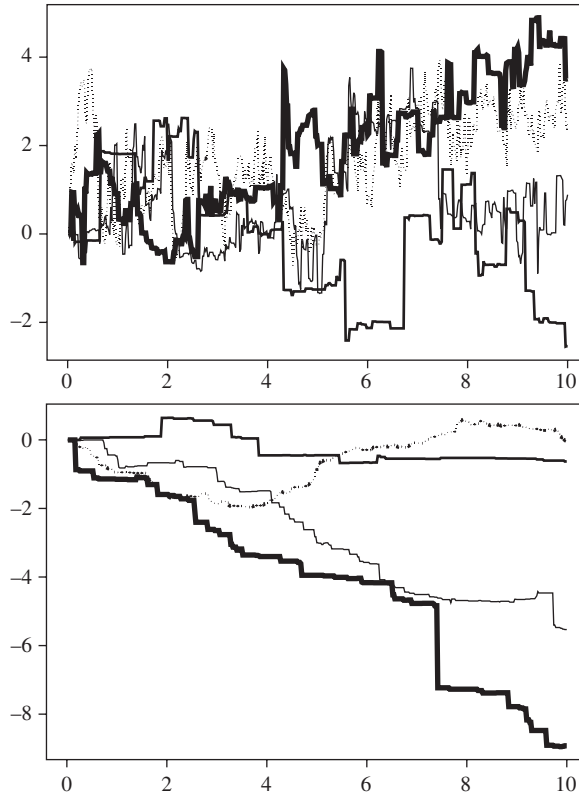
FIGURE 1: Trajectories of FLM for different values of the self-similarity parameter, H , and time scale parameter, \nu .
