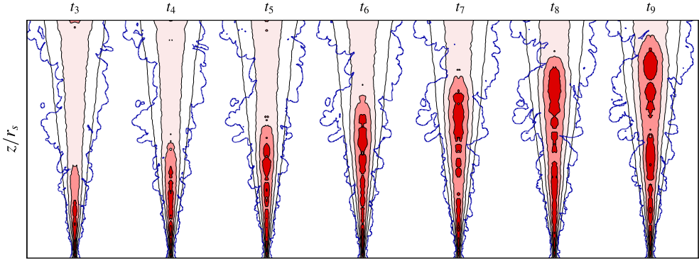
FIGURE 2. (Colour online) Isoregions of the ensemble and azimuthally averaged buoyancy (red) and threshold of the instantaneous enstrophy (blue) in an unsteady turbulent plume at times t_n \approx 1.95\tau_s n , n = 3, \dots, 9 , where \tau_s \equiv r_s^{4/3} (F_s^A)^{-1/3} . The buoyancy displayed in the figure has been non-dimensionalised using the local characteristic buoyancy scale b_{m0} \equiv B_0 M_0 / Q_0^2 of a steady plume with buoyancy flux F^B .
