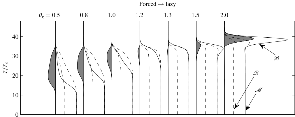
FIGURE 11. Wave structure for different values of \theta_g . The dashed lines are normalised integral quantities \mathcal{Q} \equiv Q/Q_0 , \mathcal{M} \equiv M/M_0 and the solid line is \mathcal{B} \equiv B/B_0 . The shaded region denotes the extent to which \Gamma(z, t) is different from unity. For \theta_g \approx 4/3 , \Gamma = 1 and the wave is pure.
