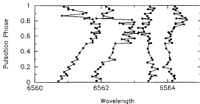
Figure 1. Wavelength associated with the H\alpha blue, central and red components. Also reported (first variation on the left) is the evolution of the Fe I at 6003 \text{ \AA} line, shifted by 558 \text{ \AA} .
