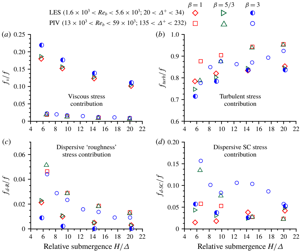
FIGURE 14. (Colour online) Dependence of the mechanism-based contributions f_v/f (a), f_{urb}/f (b), f_{d-R}/f (c) and f_{d-SC}/f (d) to the overall friction factor f on the relative submergence at intermediate (LES) and high (PIV) Reynolds numbers.
