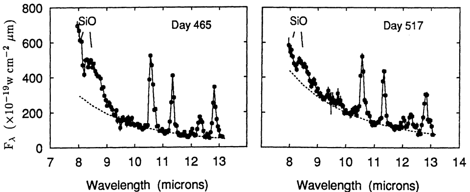
Fig 1. Spectra at 8\text{--}13 \mu\text{m} of SN 1987A 465 and 517 days after the explosion.
