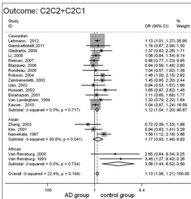
Figure 2: Forest plot of AD risk associated with rs1049296 under C2C2+C2C1 vs C1C1 contrast in different ethnicity. The squares and horizontal lines correspond to the study-specific OR and 95% CI. The area of the squares reflects the study specific weight. The diamond represents the pooled OR and 95% CI.
