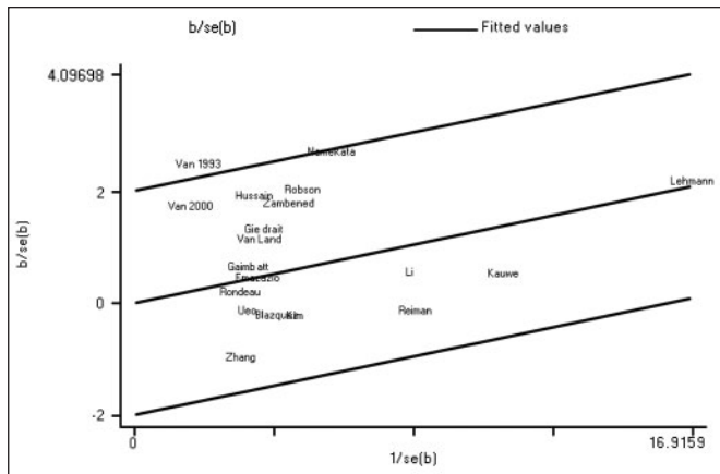
Figure 4: Galbraith plot of associations between TF gene rs1049296 polymorphisms and AD risk, produced by first dividing each estimate by its standard error (se) to generate z-statistics (b/se(b)), which is then plotted versus 1/se(b) for each of studies. Inner line represents pooled effect and outer lines represent 95% limits. Each author represents the respective study included in the meta analysis (shown in Table 1) for the indicated association by C2C2 vs C2C1+C1C1.
