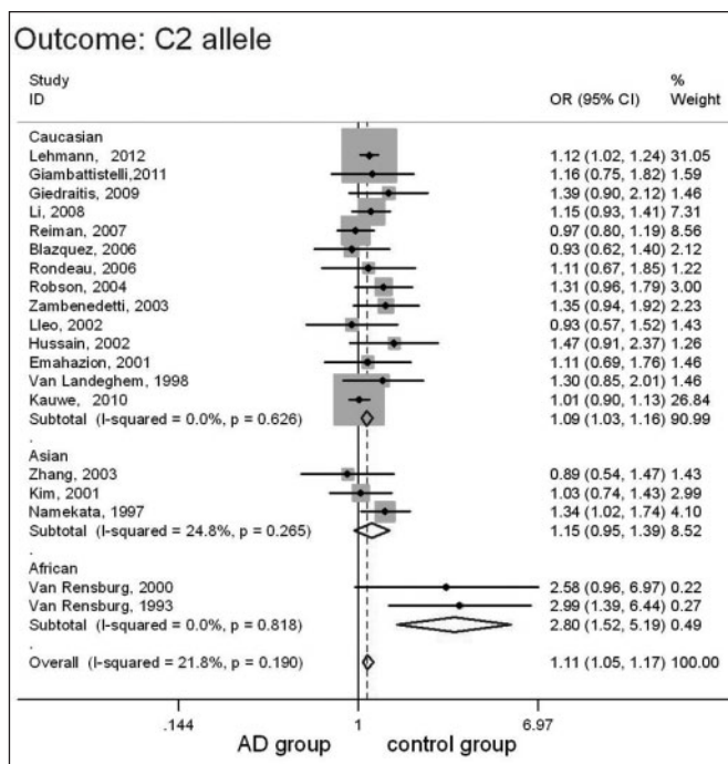
Figure 3: Forest plot of AD risk associated with rs1049296 under allele contrast C2 vs C1 in different ethnicity. The squares and horizontal lines correspond to the study-specific OR and 95% CI. The area of the squares reflects the study specific weight. The diamond represents the pooled OR and 95% CI.
