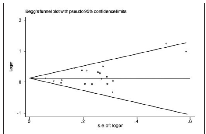
Figure 6: Begg’s funnel plot of publication bias in TF gene rs1049296 polymorphism studies. Log OR is plotted versus standard error for each of studies in this meta analysis. Each circle represents a separate study for the indicated association by C2C2 vs C2C1+C1C1.
