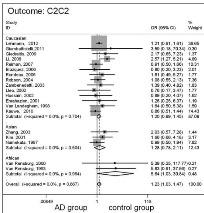
Figure 1: Forest plot of AD risk associated with rs1049296 under C2C2 vs C2C1+C1C1 contrast in different ethnicity. The squares and horizontal lines correspond to the study-specific OR and 95% CI. The area of the squares reflects the study specific weight. The diamond represents the pooled OR and 95% CI.
