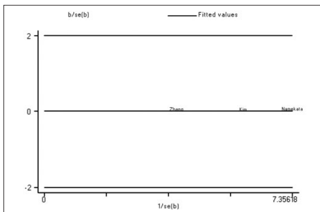
Figure 5: Galbraith plot of associations between TF gene rs1049296 polymorphisms and AD risk, produced by first dividing each estimate by its standard error (se) to generate z-statistics (b/se(b)), which is then plotted versus 1/se(b) for each of studies. Inner line represents pooled effect and outer lines represent 95% limits. Each author represents the respective study included in the meta analysis (shown in Table 1) for the indicated association by C2 vs C1.
