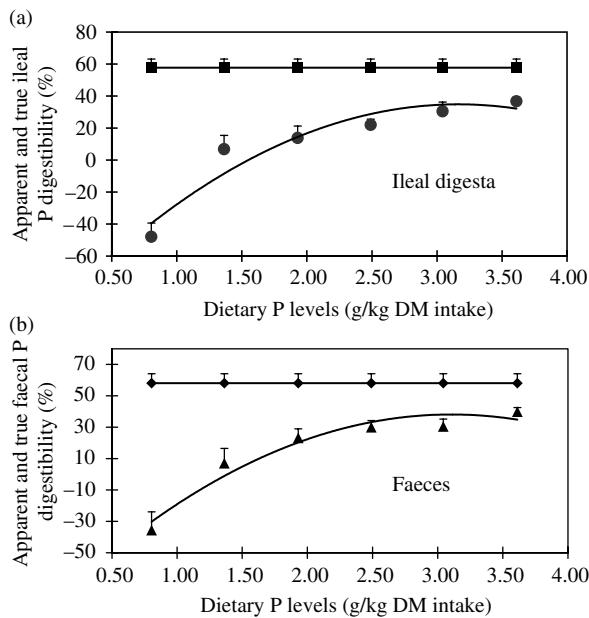
Figure 3 Effects of dietary phosphorus (P) levels [(g/kg dry matter (DM) intake) on apparent (● or ▲, %, mean \pm s.e., n = 6 , for each data point) and true (■ or ◆, %, mean \pm s.e., n = 36 , for each data point) ileal and faecal P digestibility values in weanling pigs fed brown rice-based diets containing various P levels. (a) Ileal digestibility values: the quadratic relationship between apparent ileal P digestibility values ( Y , %) and the dietary levels of P ( x , g/kg DM diet), Y = -13.36x^2 + 84.54x - 98.93 , n = 36 , R^2 = 0.77 , P < 0.05 . (b) Faecal digestibility values: the quadratic relationship between apparent faecal P digestibility values ( Y , %) and the dietary levels of P ( x , g/kg DM diet), Y = -12.91x^2 + 80.16x - 86.33 , n = 36 , R^2 = 0.75 , P < 0.05 .
