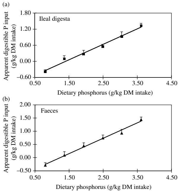
Figure 1 Linear relationships between the apparent ileal (■) and faecal (▲) digestible dietary phosphorus (P) ( y : g/kg dry matter (DM) intake, mean \pm s.e., n = 6 , for each data point) or the dietary total P levels ( x : g/kg DM intake) in weanling pigs fed the brown rice-based diets. (a) In ileal digesta: y = 0.578x - 0.812 , n = 36 , r^2 = 0.854 , P < 0.05 . (b) In faeces: y = 0.584x - 0.725 , n = 36 , r^2 = 0.869 , P < 0.05 .
