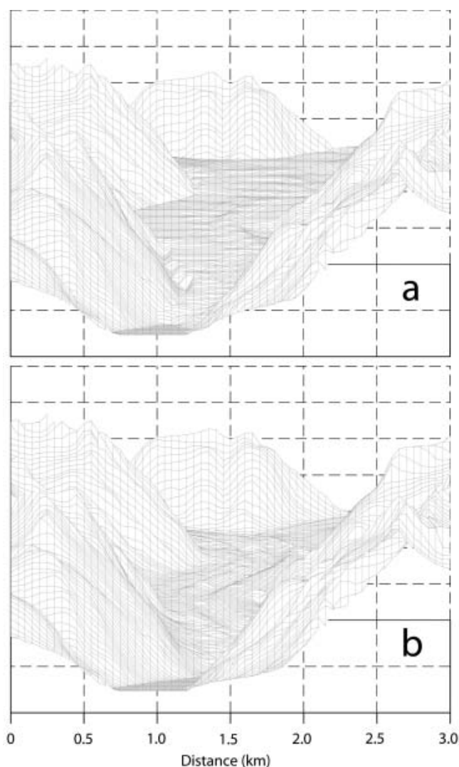
Fig. 2. DEMs of (a) the glacier surface in 1927, digitized from topographic maps (Bauder, 2001), and (b) the glacier surface in 1997, derived photogrammetrically from aerial photographs (Bauder, 2001). View is in up-glacier direction; north points to the right.
