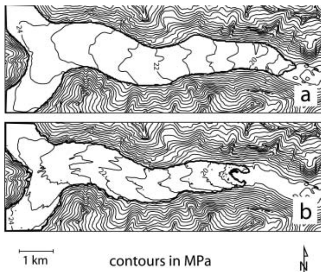
Fig. 5. Contours of equal hydraulic potential computed using k = 1 in (a) 1927 and (b) 1997.
