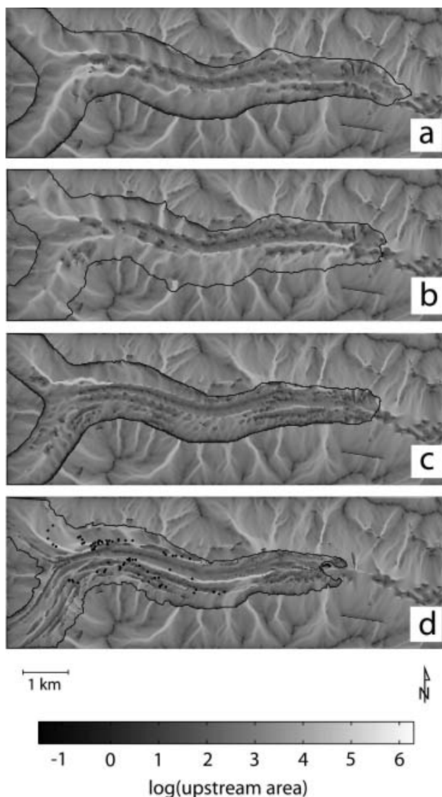
Fig. 6. Upstream area distributions computed using k = 1 in (a) 1927, (b) 1947, (c) 1961 and (d) 1997. The black dots in (d) mark the locations of active moulins surveyed and mapped in 2002 (Braun, 2003).
