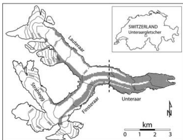
Fig. 1. Map of Unteraargletscher and its two main tributaries, Finsteraar- and Lauteraargletscher. The dashed line indicates the location of cross-sectional profiles shown in Figure 4 (see text for details). Shading on glacier represents debris-covered ice. Inset shows the study area in the Bernese Alps.
