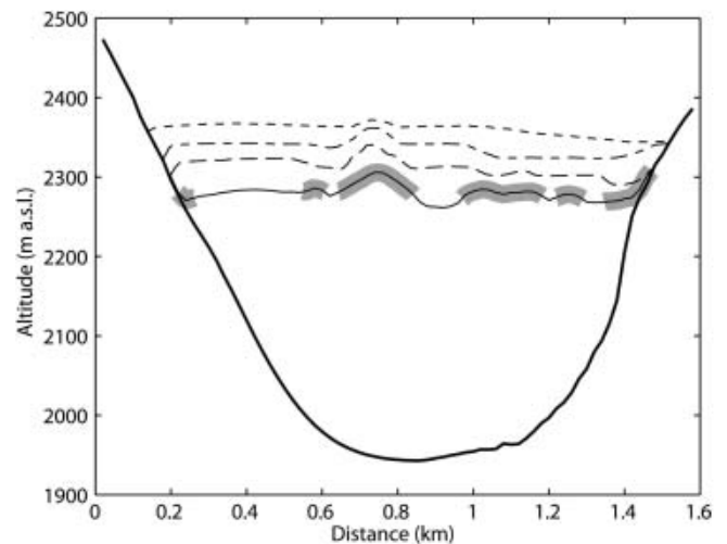
Fig. 4. Cross-sectional profiles through Unteraargletscher in 1927 (dotted line), 1947 (dash-dotted line), 1961 (dashed line) and 1997 (solid line) at the location shown in Figure 1. Note the increase in height of the medial moraines concurrent with the thinning of the glacier. Thick grey lines indicate debris-covered ice in 1997. Glacier flow is into the page; north points to the left.
