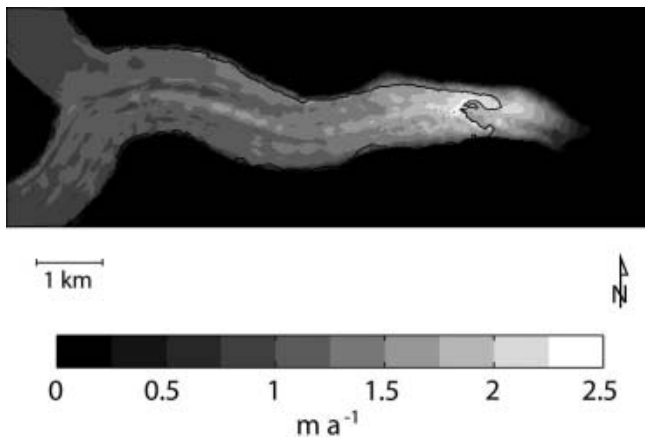
Fig. 3. Mean annual decrease in surface elevation, 1927–97. Black line shows the 1997 glacier boundary.
