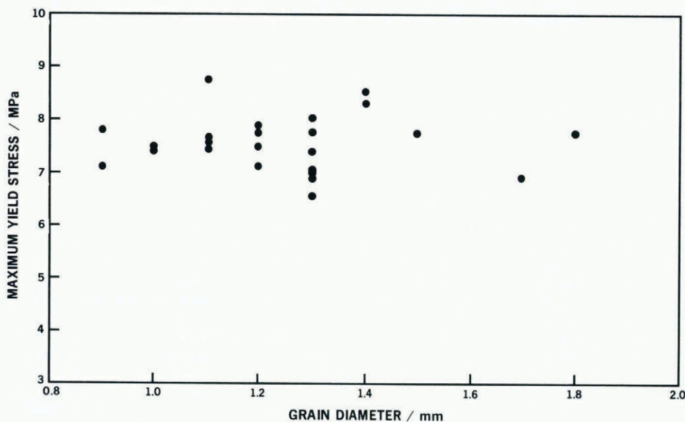
Fig. 1. The maximum yield stress plotted against grain-size, for laboratory-grown polycrystalline ice tested at -10.5^{\circ}\text{C} strain-rate 5.5 \times 10^{-4} \text{ s}^{-1} , sample diameter 20 mm, sample length 60 mm.
