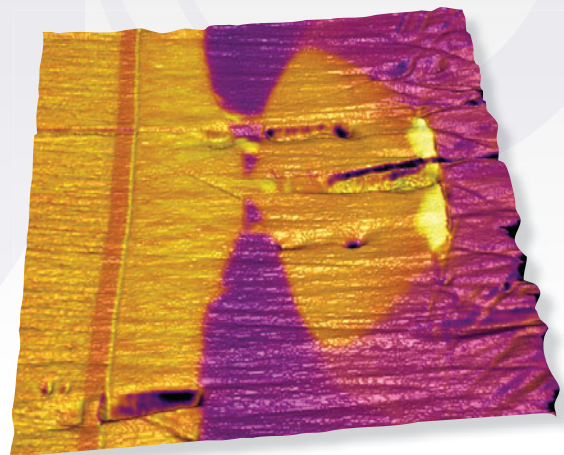
Stiffness of active region of hard disk read-write head, 6µm scan
