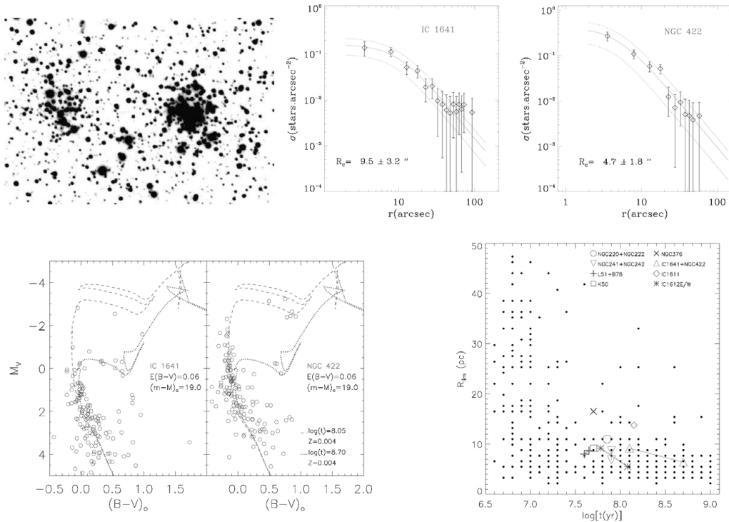
Figure 1. From top left to bottom right: (i) V image extraction ( 2.6' \times 1.7' ) of pair IC 1641 (left) / NGC 422 (right); north is up and east to the left; (ii) The RDP on a logarithmic scale with a two-parameter King-profile fit superimposed, for which R_c is indicated; 1\sigma dispersions of the fits are plotted as dotted lines; (iii) Isochrone fits to the CMDs of IC 1641 and NGC 422; for comparison, the best-matching isochrone for IC 1641 is also plotted in the CMD of NGC 422 and vice versa; (iv) Limiting radius (Bica et al. 2008) as a function of age; the dots represent SMC clusters from Chiosi et al. (2006) and other symbols identify the present sample of binary/merger clusters.
