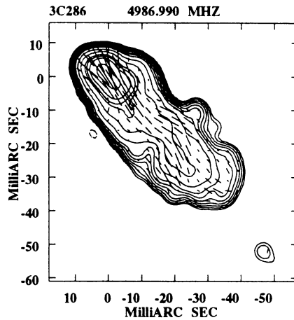
Figure 1. EVN polarization image of 3C286. Contour levels are -3.0,3.0, 4.2,6,8.4,12,16.8,24,45,90,180,240,360 and 750 mJy/beam and the peak is 1.0 Jy/beam. The vectors represent the projected orientation of the electric vector; their length is proportional to the polarized flux density.
