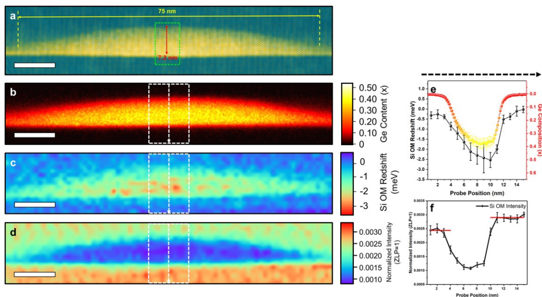
Figure 1. Figure 1: Nanoscale elemental and vibrational spectroscopy of a SiGe QD. (a) Atomic resolution high angle annular dark field image of a SiGe QD. (b) Core loss elemental mapping of a SiGe QD. (c-d) Mapping of the Si optical mode redshift and peak intensity respectively (e) Line profiles of composition (b) and redshift (c) mapping. (f) Line profile of Si optical mode intensity. scale bars are 10nm.
