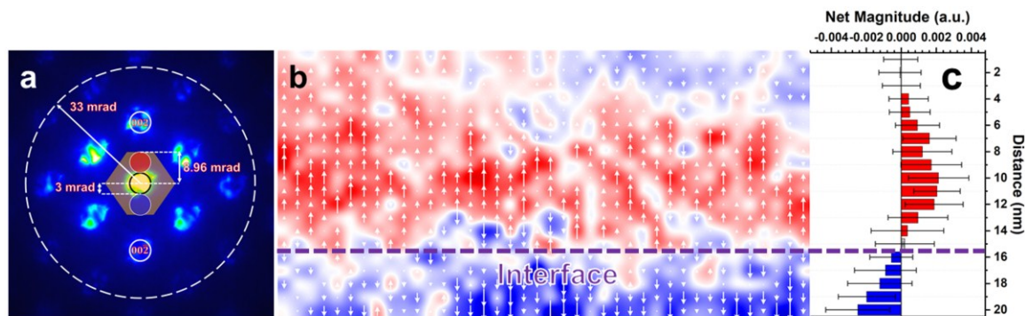
Figure 2. Figure 2: Momentum resolved differential mapping of phonon vertical momentum. (a) 3mrad convergence semi-angle diffraction pattern where the 002 and 00-2 spots are labeled. First Brillion zone of Si is marked in orange and distance to the X point is labeled. The red and blue circles near the center denote the EELS entrance aperture positions where off axis data was acquired is illustrated. (b) Differential momentum mapping from spectra acquired at the blue and red circled locations in (a). (c) Horizontally averaged line profile of (b).
