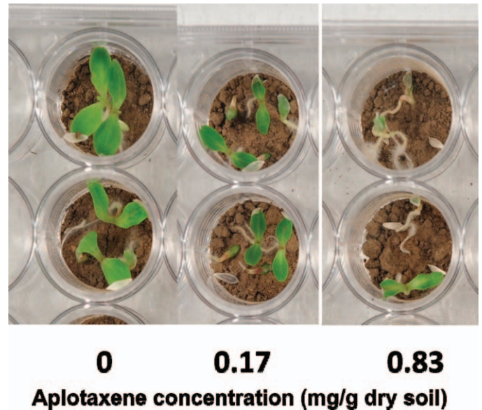
Figure 7. Effects of aplotaxene, a potential allelochemical found in high concentrations in the roots of a number of invasive species, on growth of lettuce in soil. Aplotaxene was added to the soil in acetone, allowed to dry and mixed in, and then seeds and water were added.
