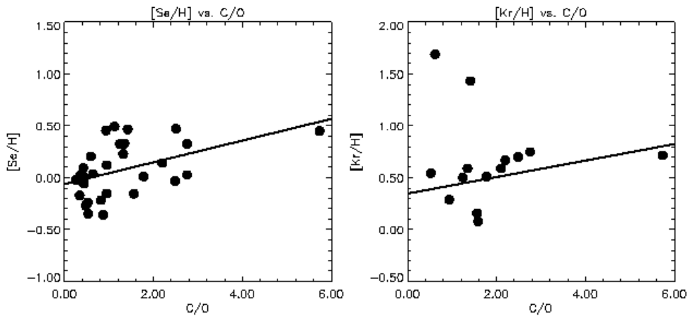
Figure 1. Se and Kr abundances vs. C/O. The solid lines are linear fits (excluding the two outliers, both Type I PNe, with high [Kr/H] and low C/O).
