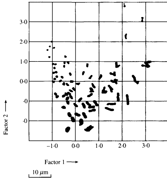
Fig. 1. Subject 7: modified scatter plot of bacteria from faecal flora: first two principal components.
