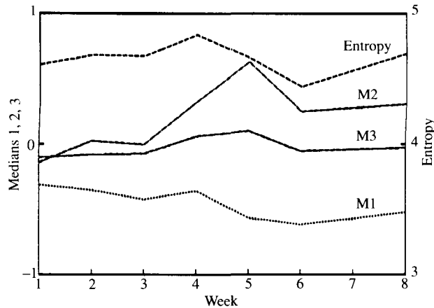
Fig. 4. Subject 1: medians of principal components 1, 2 and 3, and entropy as functions of time.
