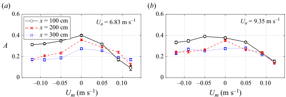
Figure 12. Variation with current velocity U_w of asymmetry A at three fetches x and wind velocity U_a values (a) 6.83 \text{ m s}^{-1} and (b) 9.35 \text{ m s}^{-1} .
