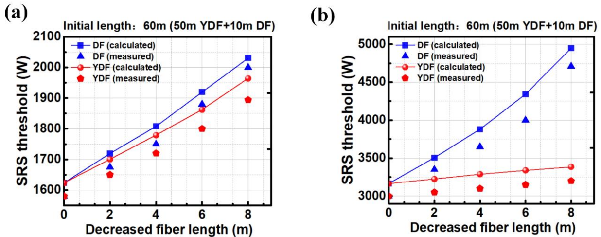
Figure 3. Experimentally measured and calculated SRS threshold versus the decreased length of DF (blue) and YDF (red) in (a) co-pumping and (b) counter-pumping scheme.
