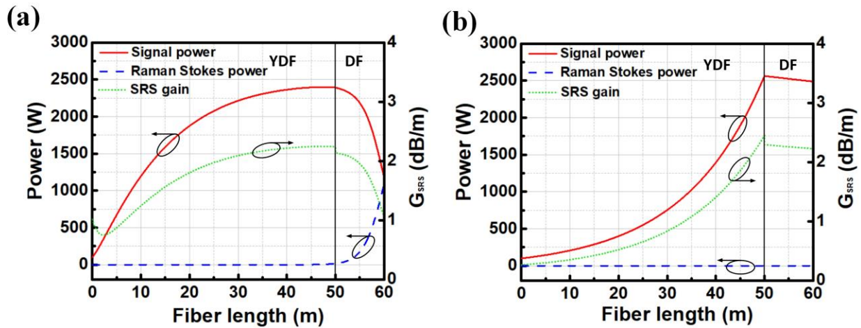
Figure 1. The evolution of signal power, Raman Stokes power and SRS gain along the fiber in (a) co-pumping and (b) counter-pumping scheme.
