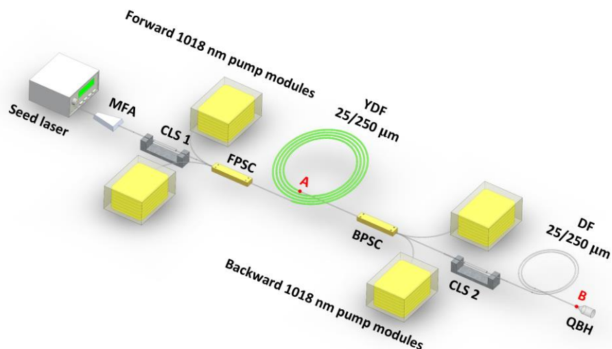
Figure 2. Experimental setup for investigating the impact of fiber length on the SRS threshold in co-pumping and counter-pumping amplifier.
