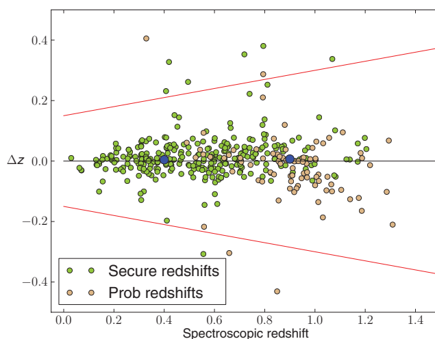
Figure 4. The deviation \Delta z between spectroscopic and photometric measures of redshift plotted against the spectroscopic redshift for objects with secure and probable spectroscopic redshifts (the green and tan circles, respectively). The median of the difference—in bins of width 0.5 in redshift, centred at z = 0.4 and 0.9 —are plotted as the large blue circles. The horizontal black line represents equality between the photometric and spectroscopic redshifts. The red lines represent the boundary beyond which the photometric redshift differs from the spectroscopic one by more than 0.15(1+z) .
