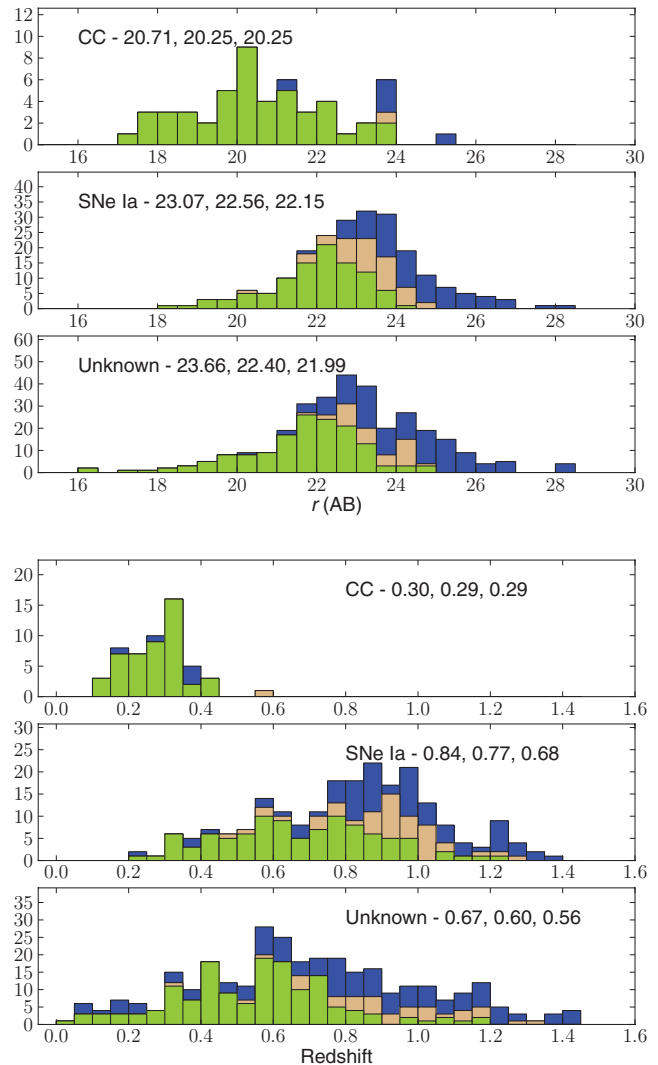
Figure 2. As for Figure 1, but split according to the photometric classification.
