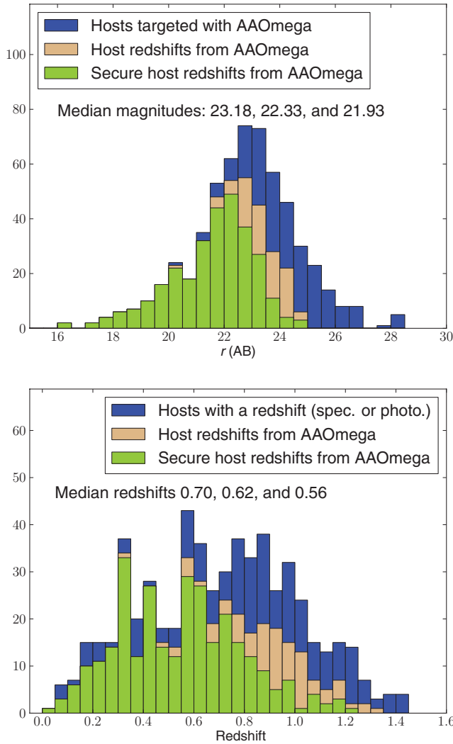
Figure 1. Histograms of the number of objects plotted as a function of magnitude (top) and redshift (bottom). The blue, green, and tan histograms represent all objects targeted with AAOmega, all objects with secure AAOmega redshifts (quality flags 4 or 5), and all objects with either a secure AAOmega redshift or a probable one (quality flags 3, 4, or 5). If the r -band magnitude of the host was unavailable, then the object was not plotted in the upper plot. If a spectroscopic redshift is not available for the lower plot, we use the photometric one. If neither a spectroscopic nor a photometric redshift were available, then the object was not plotted in the lower panel. The median magnitudes and redshifts of objects in the blue, tan, and green histograms annotate each figure.
