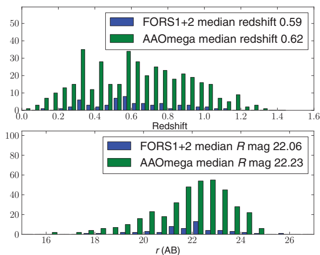
Figure 3. A comparison of the host redshift and magnitude distributions obtained with FORS1 and FORS2 with the host and magnitude distributions obtained with AAOmega.
