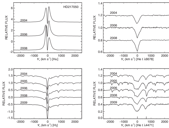
Figure 1. Example of a “quadruple plot” (this of HD 217050). In each quadrant are plots of the normalized fluxes of the seasonal averages of the spectra, offset for clarity, and in radial velocity space. Each is centered on the rest wavelength of a different spectral feature: top left - H \alpha , top right - He I \lambda 6678 , bottom left - H \gamma , and bottom right - He I \lambda 4471 (with a mark at \sim 670 \text{ km s}^{-1} delineating Mg II \lambda 4481 ).
