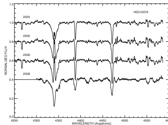
Figure 2. A plot of seasonal averages of the normalized flux versus wavelength for the blue spectrum of 31 Peg (HD 212076) - notice how all emission features diminish greatly in 2009. These spectra are offset for clarity.
