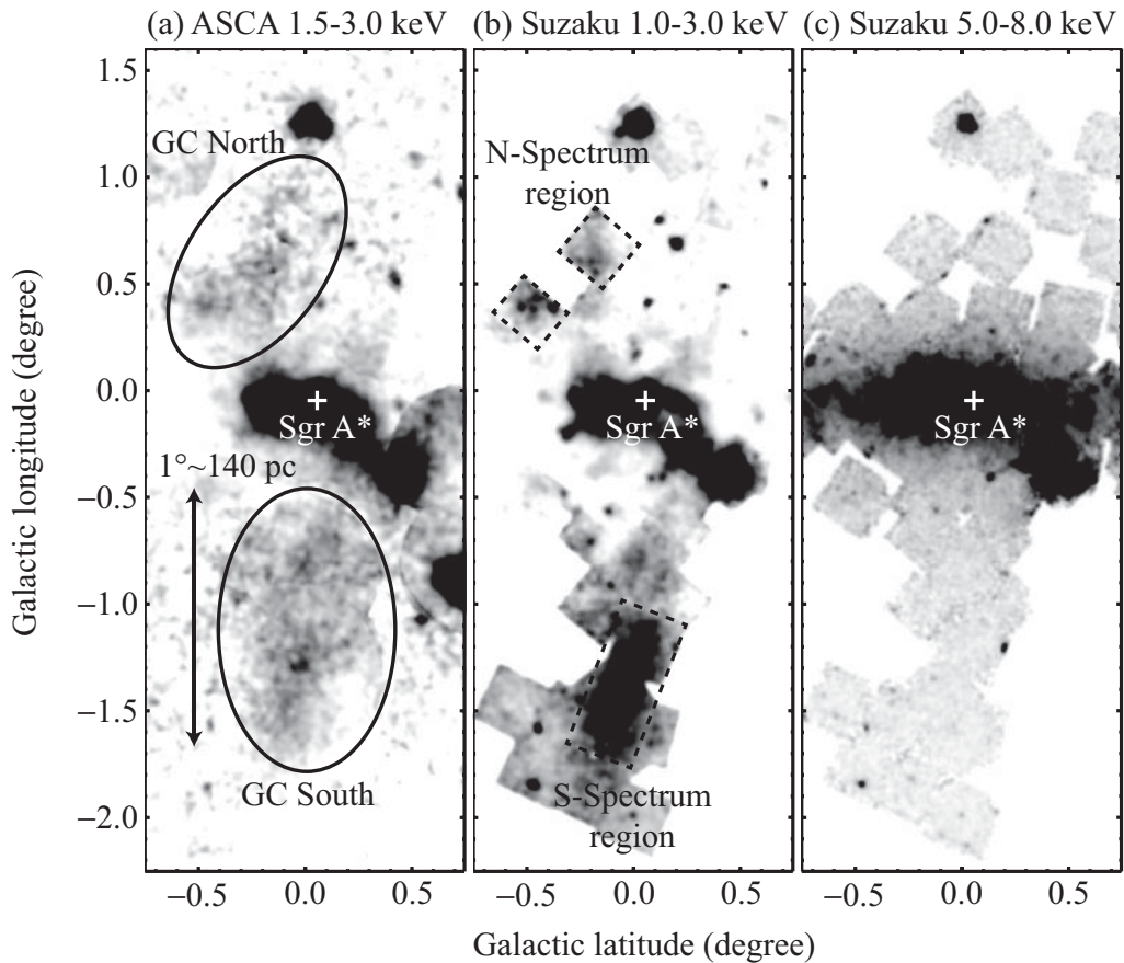
Figure 1. X-ray images of the GC in the (a) 1.5–3.0 keV band with ASCA , (b) 1.0–3.0 keV band with Suzaku , and (c) 5.0–8.0 keV band with Suzaku .
