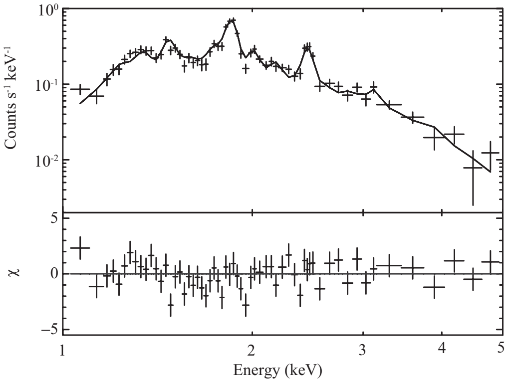
Figure 3. Spectrum of GC North fitted with the CIE plasma model.
