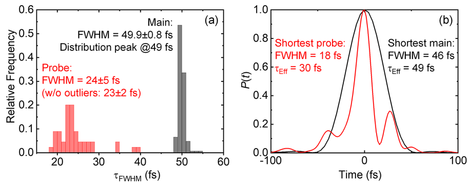
Figure 4. Stability of the probe pulse compression and the shortest measured pulses. (a) FWHM histograms for the BA1 \times 2 mode, which provides the optimum average compression. (b) Shortest main and probe pulses; the latter was obtained in the BA2 \times 1 laser shot with the main pulse energy of 4 J and probe pulse energy of approximately 5.8 mJ.
