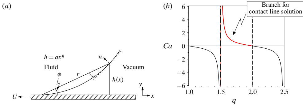
FIGURE 6. (Colour online) (a) Sketch of the cusp solution for a 180^\circ contact angle. (b) Solutions of (2.9).
