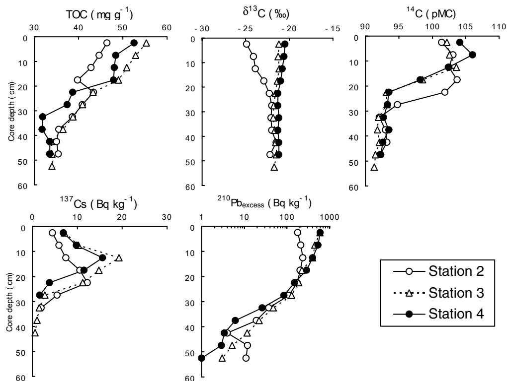
Figure 4 Vertical profiles of total organic carbon (TOC), \delta^{13}\text{C} , ^{14}\text{C} , ^{137}\text{Cs} and ^{210}\text{Pb}_{\text{excess}} in core sediment samples at Stations 2, 3, and 4 from Lake Obuchi. Profile data of ^{137}\text{Cs} and ^{210}\text{Pb}_{\text{excess}} are from Ueda et al. (2004b).
