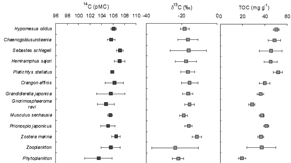
Figure 3 ^{14}\text{C} activity, \delta^{13}\text{C} , and TOC (total organic carbon) in aquatic biota from Lake Obuchi
