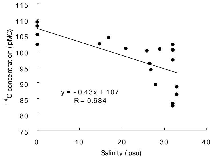
Figure 2 Relationship between ^{14}\text{C} activity and salinity in the water samples
