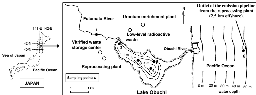
Figure 1 Sampling locations for Futamata River, Lake Obuchi, and the Rokkasho coast, Japan
