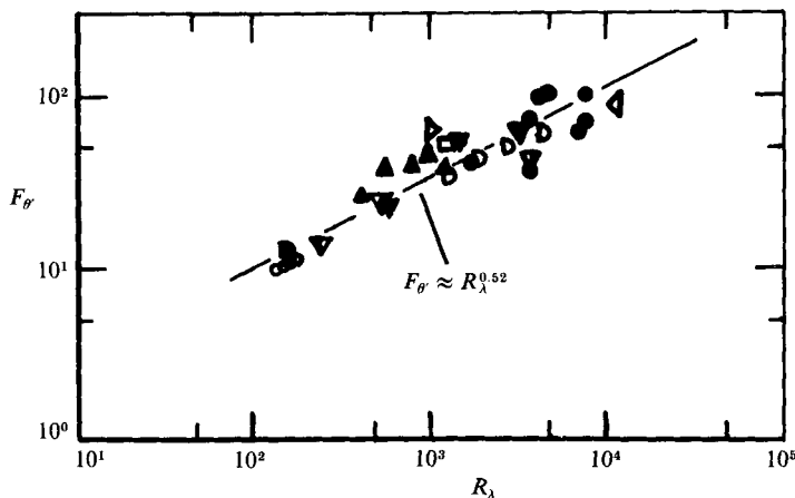
FIGURE 17. The kurtosis of the temperature derivative (dT/dt) . \bullet , McConnell (1976), atmosphere; \triangleleft , Antonia et al. (1980), atmosphere; \mathcal{D} , Antonia & Danh (1977), atmosphere; \circ , Sreenivasan, Antonia & Danh (1977), boundary layer; \blacktriangle , Gibson et al. (1970), atmosphere; \triangleright , Park (1976), atmosphere; \square , McConnell (1976), jet; \blacktriangledown , Antonia & Van Atta (1975); \blacklozenge , Antonia & Danh (1977), jet; \blacktriangledown , Gibson & Masiello (1972), jet; \blacktriangledown , Gibson et al. (1970), jet.
