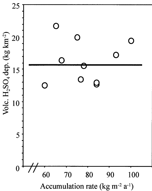
Fig. 4. Spatial distribution of volcanic sulphate deposition on Amundsenisen. The total volcanic sulphate deposition of the years 1992 and 1993 is plotted vs the snow accumulation rate.
