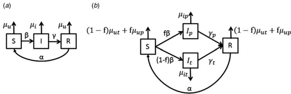
Fig. 2. Flow diagrams of epidemic models. (a) In the one-group model, three states were included: susceptible (S), infectious (I) and immune (R). (b) In two-group model, four states were included: susceptible (S), persistently infectious ( I_p ), transiently infectious ( I_t ) and immune (R). Unlike the one-group model that included only one infectious state, the two-group model included two infectious states, and bats go through either a persistently infectious state or a transiently infectious state. The two infectious states have different recovery rates, in which the recovery rate ( \gamma_p ) of a persistently infectious state is lower than the recovery rate ( \gamma_t ) of a transiently infectious state. \beta : transmission rate, \gamma : recovery rate, \omega : waning rate of immunity, \mu : mortality rate, f : proportion of recaptured bats with persistent infection to the recaptured bats with persistent or transient infection. Subscripts p, t, u and i denote ‘persistent infection’, ‘transient infection’, ‘uninfectious state’ and ‘infectious state’, respectively.
