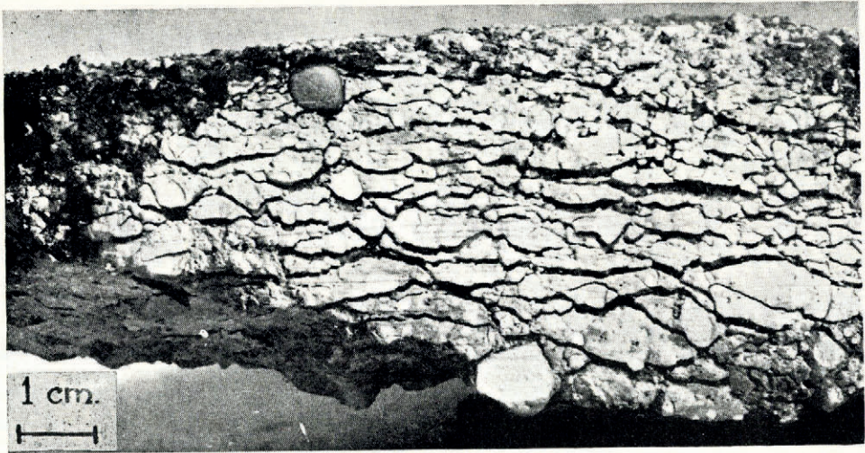
Fig. 1. Frost heaving in chalk at Saffron Walden, February 1947. The black fissures are solid ice; all the white chalk fragments were originally in close contact with each other. Many fragments have been fractured during the frost
