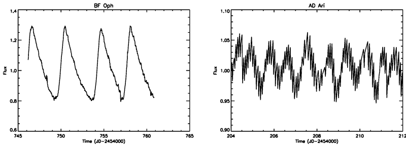
Figure 5. Left: BF Oph - Classical Cepheid - V_{\text{mag}} = 7.37 . Right: AD Ari - \delta Scuti - V_{\text{mag}} = 7.43
