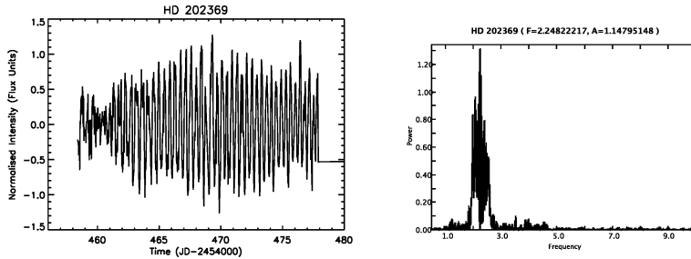
Figure 7. Left - STEREO light curve of HD 202369 which is previously suspected to be a variable. Right panel contains the power spectrum with the broad peak around the prominent period.
