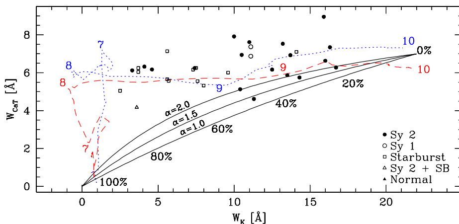
Figure 1. Comparison between nuclear W_{\text{CaT}} and W_K for our objects. We show the evolutive paths for simple stellar populations with two metallicities: 1 (dotted line) and 2.5 Z_\odot (dashed line). The numbers at those lines indicate \log(\text{age}) . The solid curves show the dilution of the equivalent widths due to a featureless power-law F_\nu \propto \nu^{-\alpha} . We found that W_{\text{CaT}} is nearly constant, thus it cannot be directly used as a stellar population diagnostic tool. We also show that the combination of W_{\text{CaT}} and W_K is inconsistent with a non-stellar featureless continuum. Purely stellar models, on the other hand, reproduce the observed values quite well.
