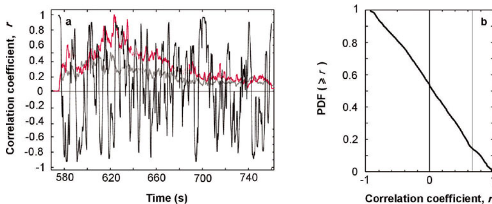
Fig. 12. Avalanche 8448. (a) Correlation of pressure signals measured by piezoelectric and cantilever sensors at 2.5 m height (black curve). The impact-pressure measurements from piezo sensors (gray curve) and cantilever sensors (red curve) are superimposed on an arbitrary scale. (b) Relative cumulative frequency distribution (PDF) of the correlation coefficient between measurements. Pressure signals are weakly correlated, with only 15% of data showing r > 0.63 .
