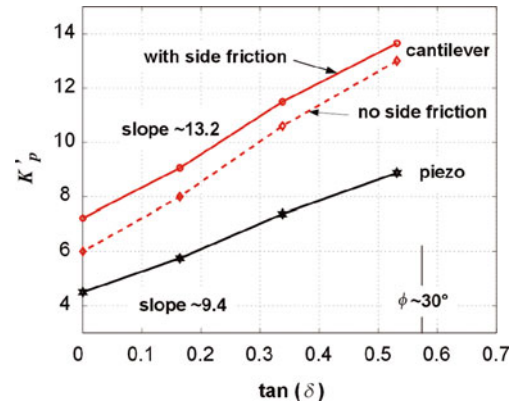
Fig. 17. Effects of Coulomb sliding friction coefficient on values of local HPEP.
