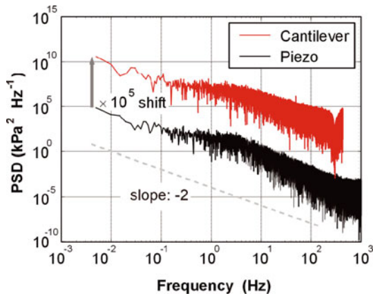
Fig. 13. Avalanche 8448. Power spectra density (PSD) of impact pressure at 2.5 m computed over the entire avalanche duration. The cantilever powder spectrum is shifted vertically by 10^5 for better legibility. The frequency dependence is shown by the gray line with a slope of -2 .
