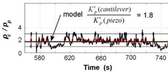
Fig. 11. Observed ratio of impact pressures (cantilever over piezo), p_c/p_p , vs time for avalanche 8448 at 2.5 m for the whole avalanche duration. The horizontal black line is the ratio predicted by the model.
