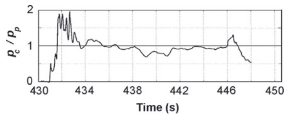
Fig. 5. Observed ratio of impact pressures (cantilever over piezo), p_c/p_p , vs time for avalanche 2009-003 at 1.5 m for the whole avalanche duration. There are two distinct regimes with a ratio of \sim 1.5 – 2.0 in the head and 1.0 in the body and tail of the avalanche.
