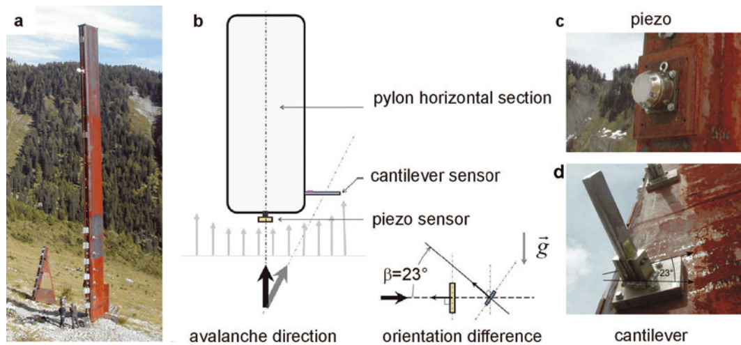
Fig. 1. (a) View of the 20 m high pylon instrumented with the two types of sensor. (b) Pylon section indicating the positions of the sensors and the 23° difference in orientation between the two types of sensor. (c) View of a piezoelectric load cell set up on the uphill face of the pylon. (d) View of a strain-gauge cantilever sensor set up on the side of the pylon.
