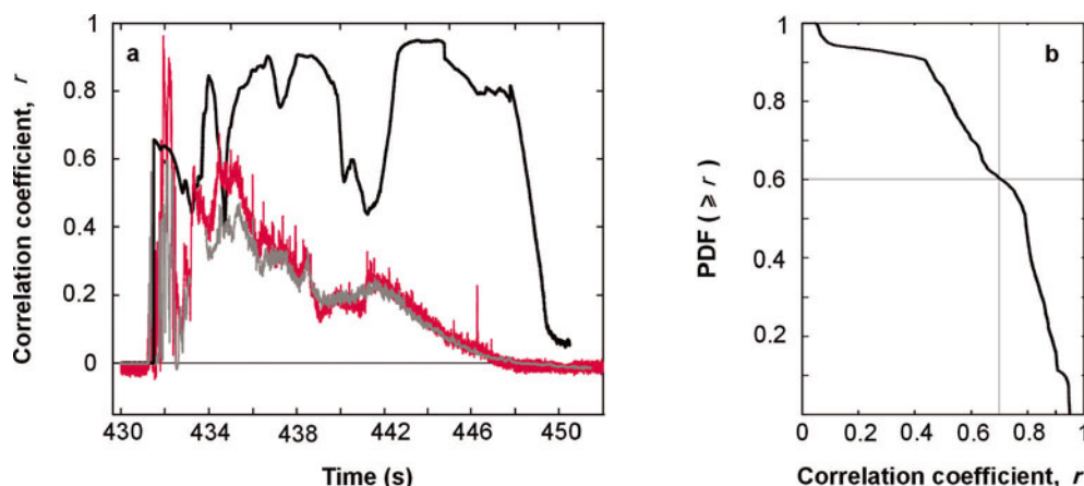
Fig. 6. Avalanche 2009-003. (a) Correlation of pressure signals measured by piezoelectric and cantilever sensors at 1.5 m height (black curve). The impact-pressure measurements from piezo sensors (gray curve) and cantilever sensors (red curve) are superimposed on an arbitrary scale. (b) Relative cumulative frequency distribution (PDF) of the correlation coefficient. Pressure signals are well correlated, with 60% of data showing r > 0.7 .
