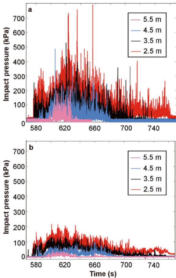
Fig. 8. Avalanche 8448. Impact-pressure raw data measured at different heights along the pylon with no orientation correction: (a) cantilever sensors; (b) piezo sensors.
