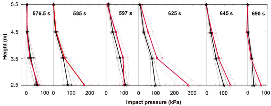
Fig. 10. Avalanche 8448. Impact-pressure profiles along the pylon height, h , at characteristic times (see Fig. 9) from piezo-electric (black lines and stars) and cantilever (red lines and dots) sensors. Error bars show one standard deviation.
