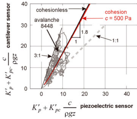
Fig. 16. Normalized horizontal pressure for cantilever vs piezo measurements (gray scattering points) using z=3 m (as estimated from pressure profiles in Fig. 10) and \rho=400 kg m -3 . Model results are given by the continuous black line with a slope of \sim 1.8 for \mu=0.4 .
