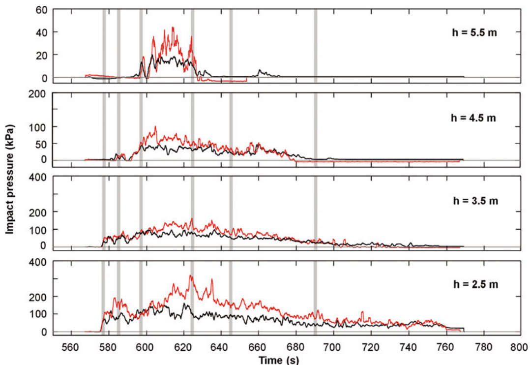
Fig. 9. Avalanche 8448. Time-averaged impact pressures along the pylon height using T=1 s for the time averaging. The red curves are the cantilever sensor pressures, and black curves are the piezoelectric sensor pressures. Vertical gray bars show characteristic times for which vertical profiles of pressure are plotted in Figure 10.
