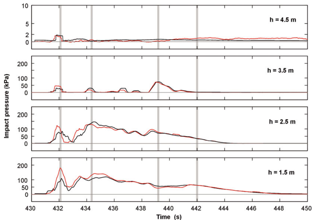
Fig. 3. Avalanche 2009-003. Time-averaged impact pressures along the pylon height using T=0.5 s for the time averaging. The red curves are the cantilever sensor pressures and the black curves are the piezoelectric sensor pressures. Vertical gray bars show characteristic times for which vertical profiles of pressure are plotted in Figure 4.
