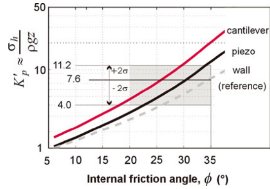
Fig. 15. Local passive earth pressure coefficients for the cantilever and piezoelectric sensors and for the wall reference case. For the cantilever sensors, the curve is computed using the parameter \delta/\phi = 2/3 which leads to values for Coulomb friction coefficient \mu \sim \tan \delta in the range \sim 0.30 – 0.45 in accordance with observations by Platzer and others (2007a,b) for \phi in the range \sim 20 – 35^\circ . The gray box vertical extension is in the range 4.0 – 11.2 as reported by Sovilla and others (2010).
