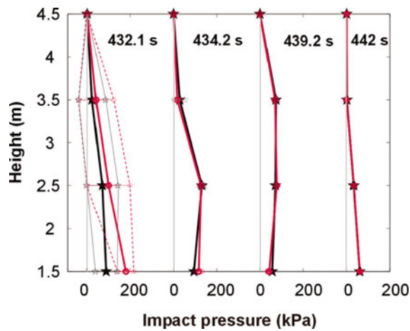
Fig. 4. Avalanche 2009-003. Impact-pressure profiles along the pylon height, h , at characteristic times (see Fig. 3) from piezo-electric (black lines and stars) and cantilever (red lines and dots) sensors. Error bars show one standard deviation.
