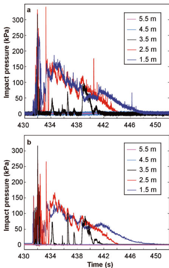
Fig. 2. Avalanche 2009-003. Impact-pressure raw data measured at different heights along the pylon with no orientation correction: (a) cantilever sensors; (b) piezo sensors.
